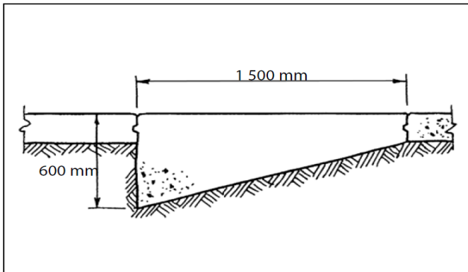
Figure 5: Anchor block
